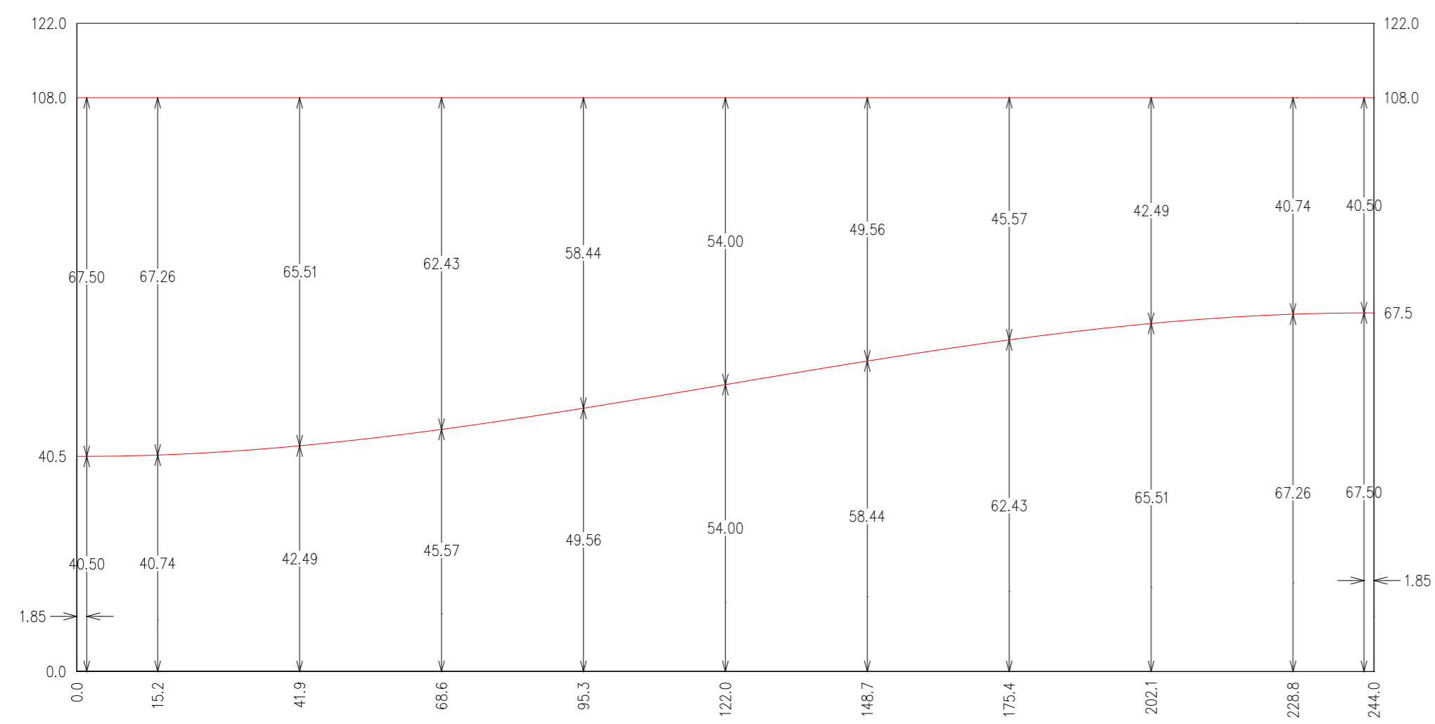
Offsets for cut lines
